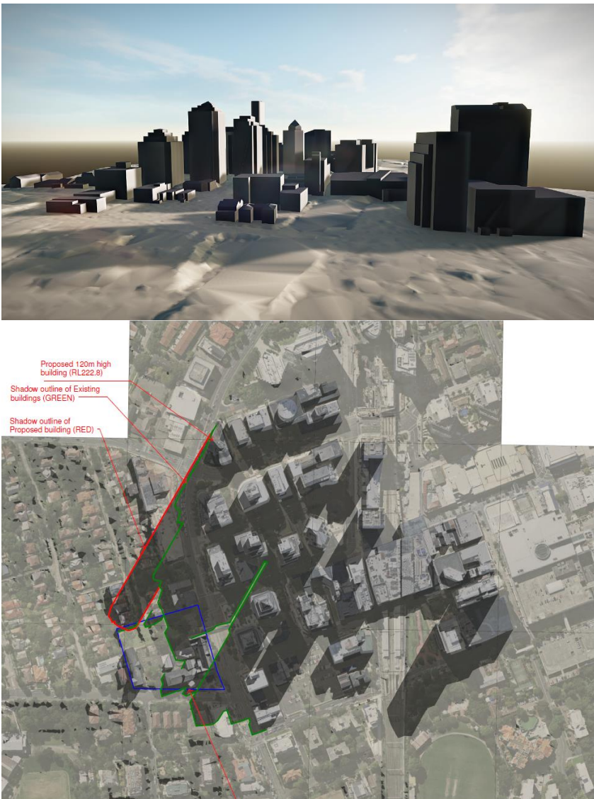
Solar Study / Rights of Light
